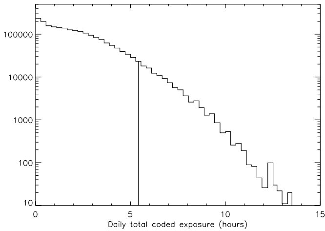
Figure 6. Histogram of the daily total coded exposure for sources detected in the BAT transient monitor. 95% of the exposures are less than 5.4 \text{ hr day}^{-1} (indicated by the vertical line.).
